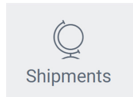
Figure 4: Shipment icon
